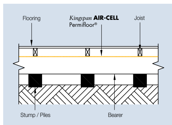
Figure 4 Side elevation of Kingspan AIR-CELL Permifloor® in a suspended framed floor
