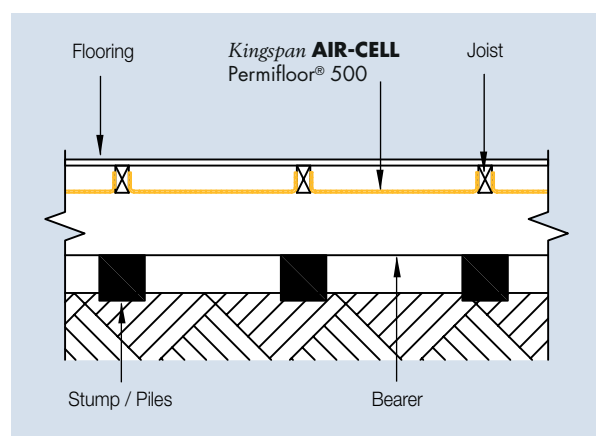
Figure 3 Side elevation of Kingspan AIR-CELL Permifloor® 500 in a suspended framed floor
