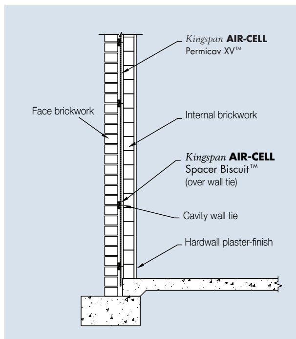
Figure 2 Side elevation of Kingspan AIR-CELL Permicanv XV™ in double brick cavity wall
