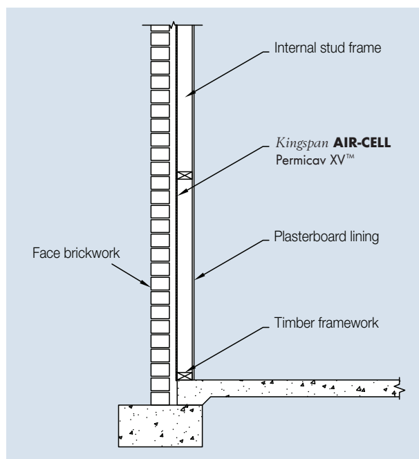
Figure 4 Side elevation of Kingspan AIR-CELL Permican XV™ in brick veneer wall
